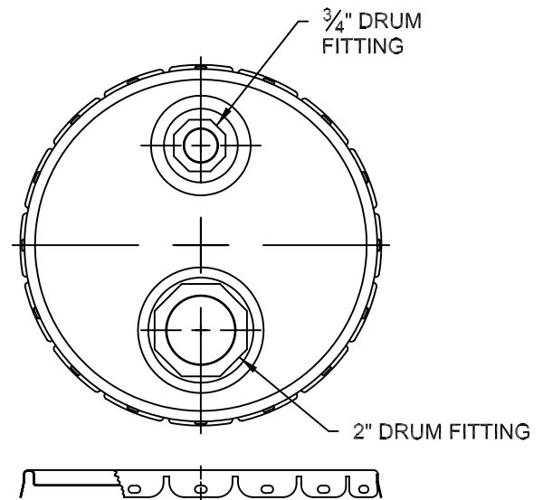
Drum Fittings:
